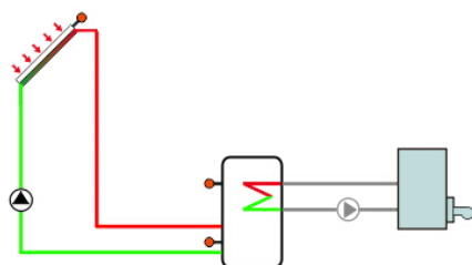
Back-up heating
